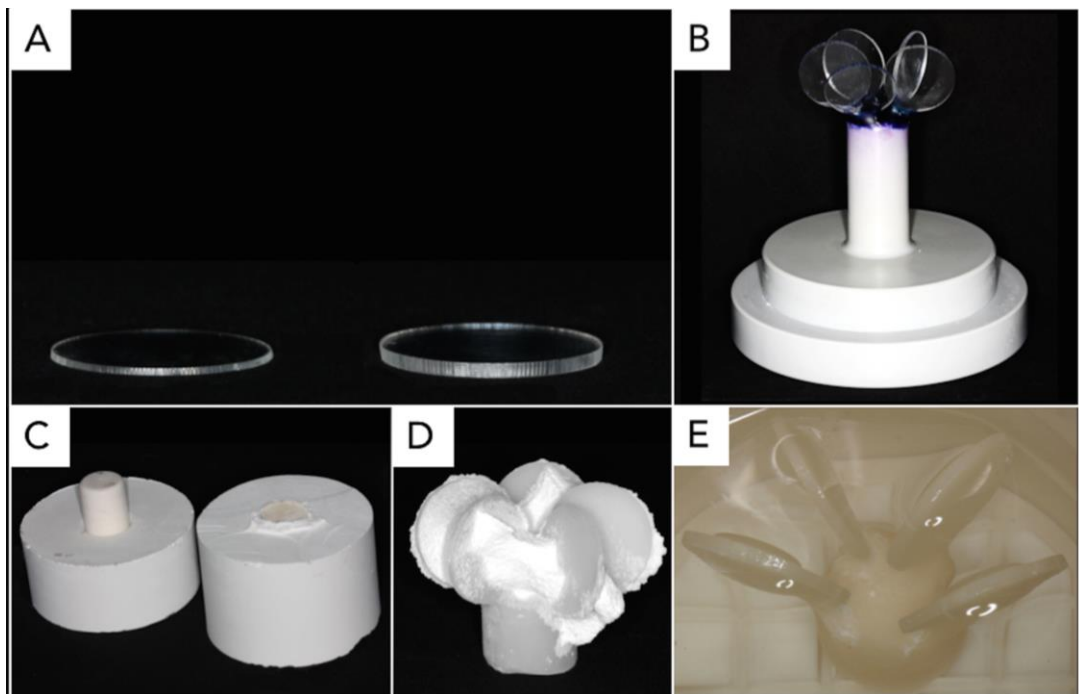
Fig. 1: Plastic sheets with thicknesses of 0.5 mm and 1.0 mm and diameter of 15 mm (A). Plastic sheets were attached to a ring mold with sprue (B). Investment was removed with a carbide disc (C). Remaining investment was sandblasted with aluminum oxide (D) and ultrasonically cleansed with IPS Invox Press liquid (E).
