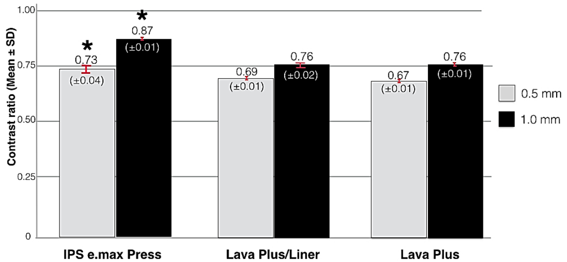
Fig. 2: Graph showing mean contrast ratio values for all ceramic specimens
