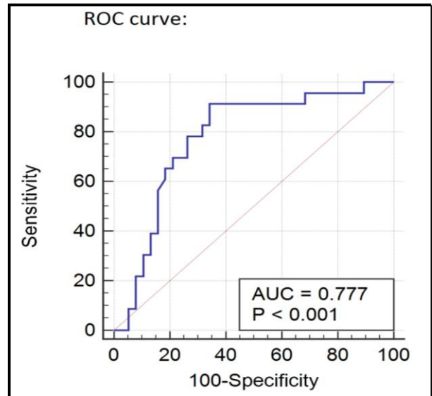
Fig. 2: The Receiver operating characteristic curve (ROC) constructed from calculations of BUN/Alb ratio as predictor of ICU need inpatients with CAP. The area under the ROC curve: 0.777 (95% CI: 0.653 to 0.874) ( p < 0.001 )
