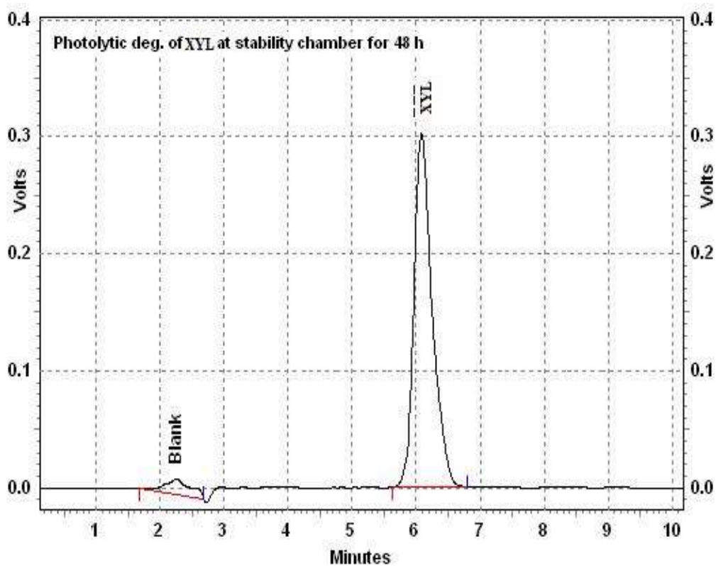
Fig. 8: Chromatograms of photolytic degradation XYL after 48 hrs
