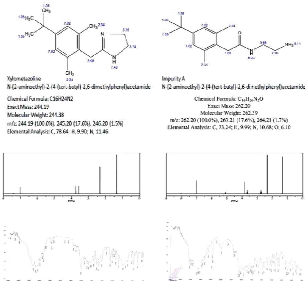
Fig. 9: Structural characterization of Xylometazoline and Impurity A by NMR, MS and IR data
