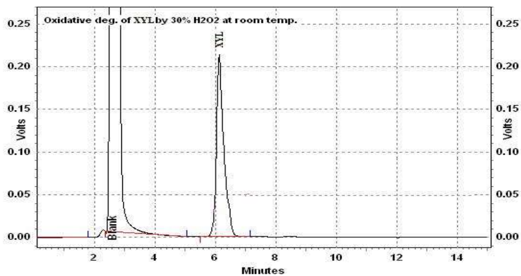
Fig. 6: Chromatograms of oxidation of XYL in 30 % H 2 O 2 after 48 hrs
