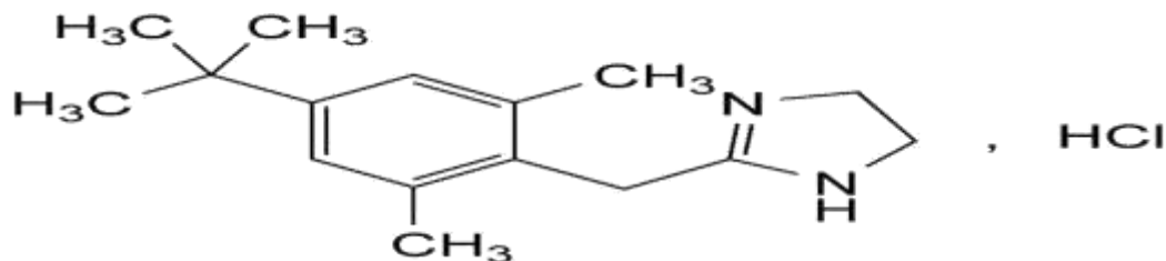
Fig. 1: Chemical structure of XYL
