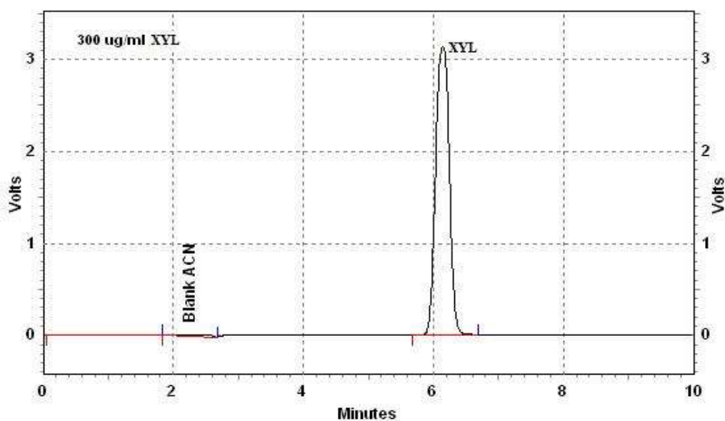
Fig. 2: Single Peak of XYL by HPLC method
