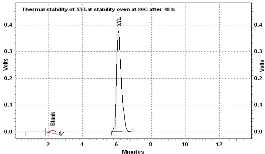
Fig. 7: Chromatograms of thermal degradation of XYL after 48 hrs
