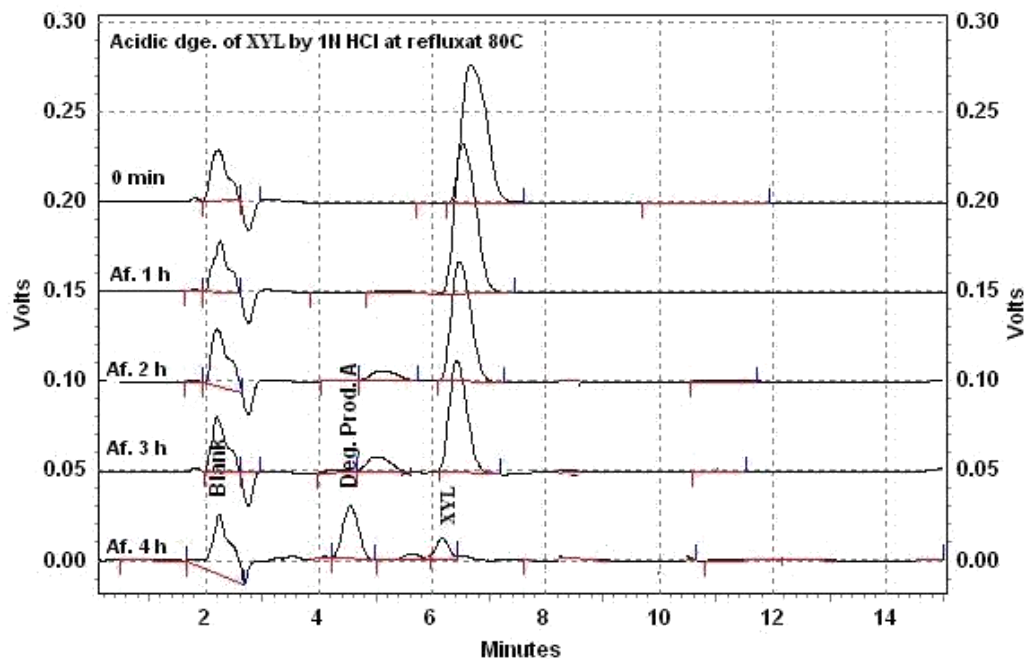
Fig. 3: Chromatograms of XYL in 1 N HCL at 0 min, after 1 hrs, 2 hrs and 3 hrs. after 4 hrs at reflux at 80 °C
