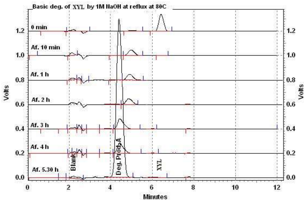
Fig. 4: Chromatograms of XYL in 1N NaOH at 0 min, 10 min after 1 hr, 2 hr, 3 hr, 4 hr and after 5.30 hrs reflux at 80 °C
