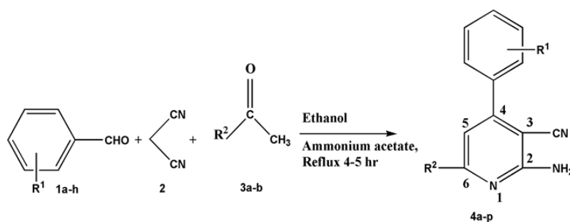
Figure 1. Multi-component synthesis of 4, 6-disubstituted-3-cyano-2-aminopyridines 4a-p .
