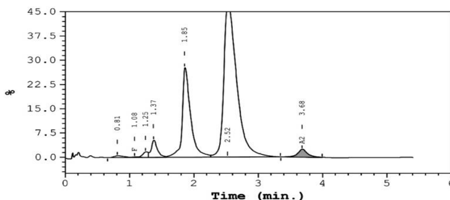
Figure 1: Showing P3 peak in HPLC
