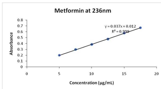
Fig. 5: Calibration curve of Metformin at 236nm
