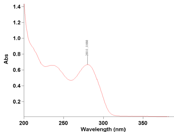
Fig. 2: Tenofovir alafenamide fumarate UV spectrum
