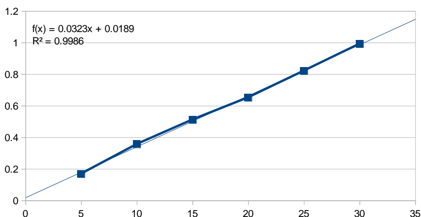
Fig. 3: Tenofovir alafenamide fumarate calibration plot
