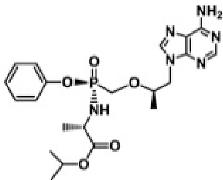
Fig. 1: Tenofovir alafenamide fumarate chemical structure
