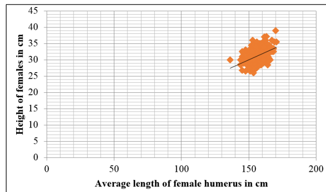
Fig. 2: Correlation of length of female humerus and height in cms: (Scatter Diagram)
