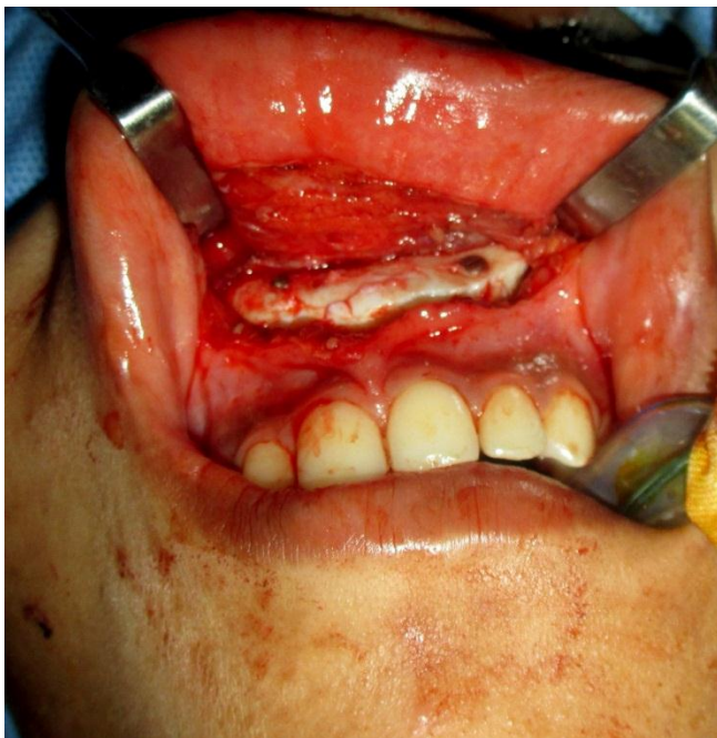
Fig. 3: Intra-operative picture showing, the screw fixation of the costochondral cartilage graft to the premaxilla.
